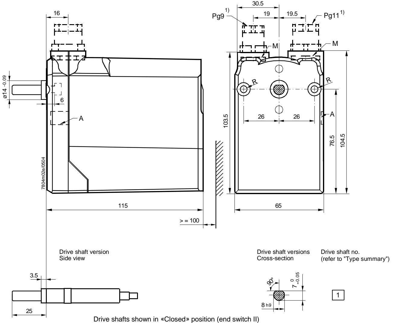
Drive shafts shown in «Closed» position (end switch II)
