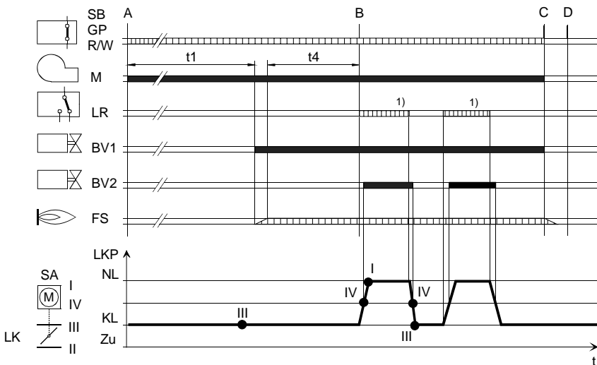
Program sequence without oil preheater
